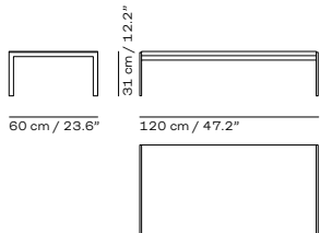
COFFEE TABLE Design: Poul Kjærholm, 1968 Tabletop: Slate, marble or granite Base: Satin-brushed stainless steel
