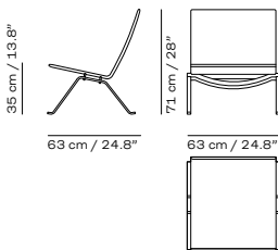
LOUNGE CHAIR Design: Poul Kjærholm, 1952 Seat: Wicker Base: Satin-brushed stainless spring steel
